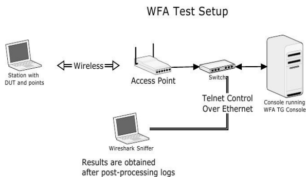
Fig 1: WFA Test Setup
