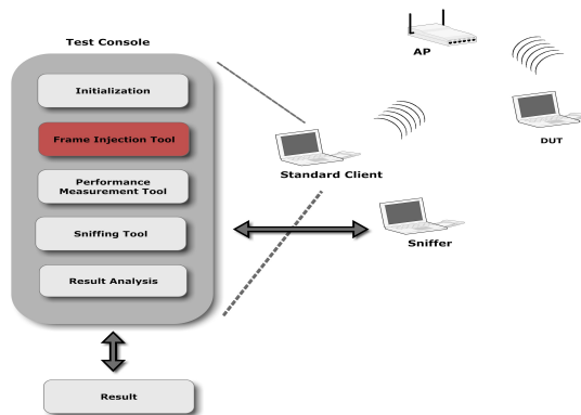
Fig 2: W-meter Components
